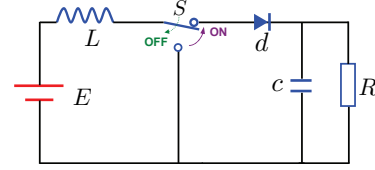
Fig. 3. The boost converter
