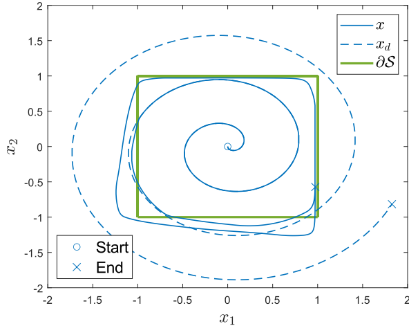
Figure 3. Trajectory of the closed-loop system in the example of Section V using a pretrained DNN but without the RISE-based disturbance observer. Since the DNN estimate is imperfect, the trajectory is allowed to leave the safe set.
