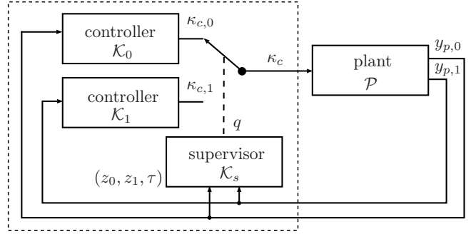
Fig. 1. Proposed control approach for Problem ( \star ).
