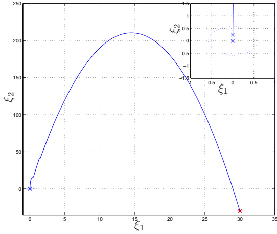
(a) Plant trajectory and zoom around origin
