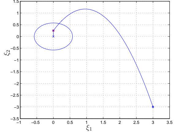
(a) Plant trajectory
