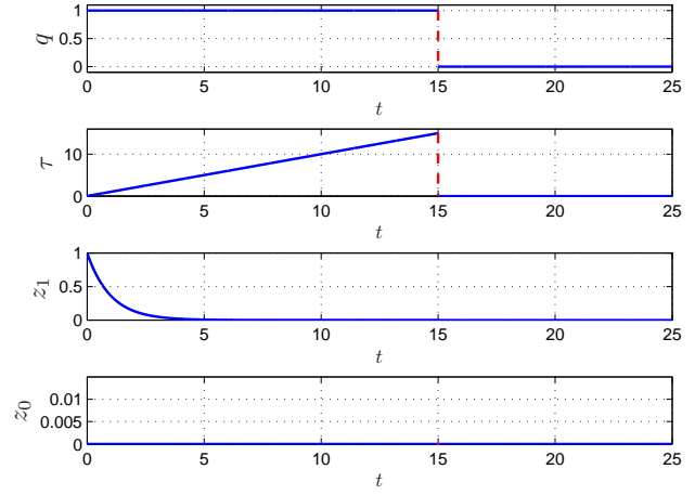
(b) Controller trajectory
